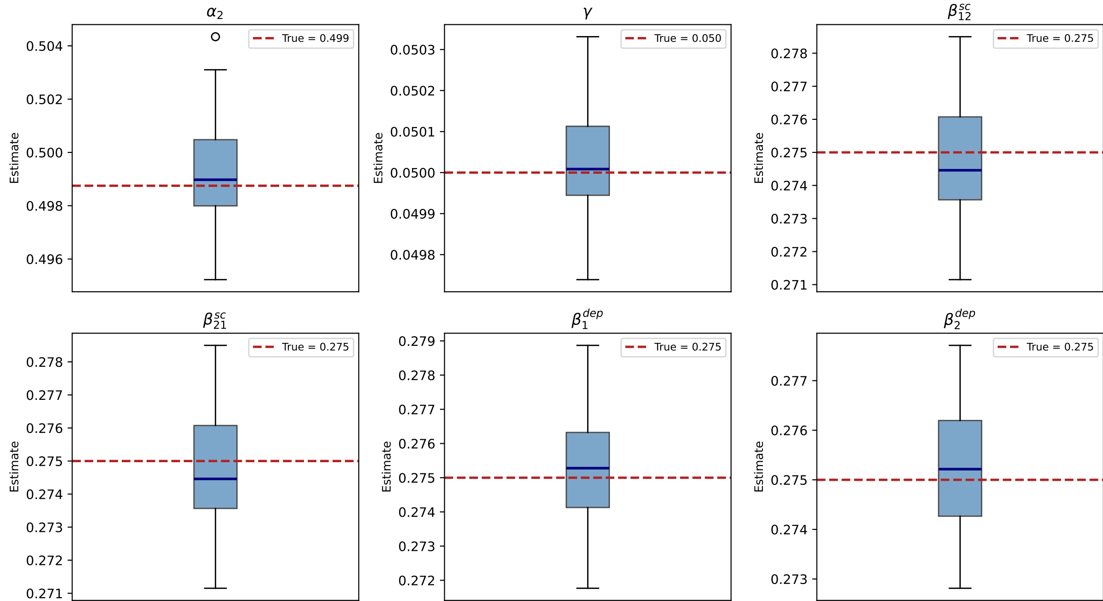
NFXP Monte Carlo: original model, symmetric switching-cost normalization (reps=50, N=50000, T=52)
